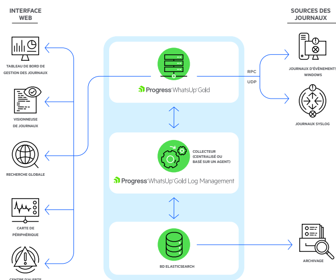
Architecture WhatsUp Gold Log Management
